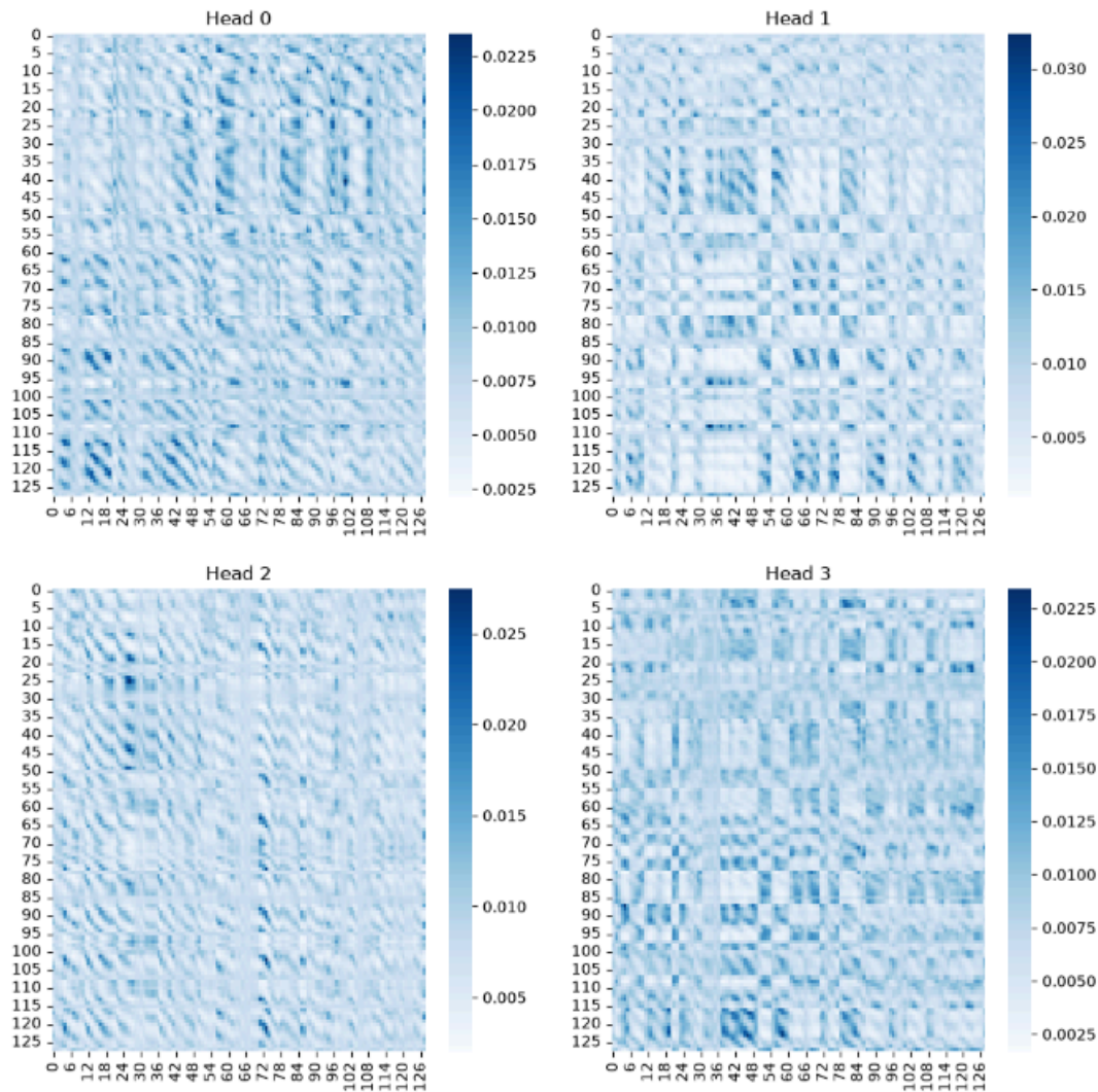
Layer 0 Attention Heatmaps (Eyes Open State)
